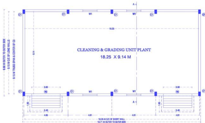
CLEANING & GRADING UNIT PLANT PLAN
