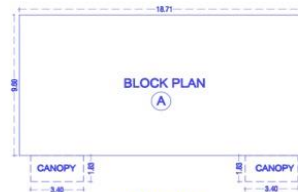
BLOCK PLAN
